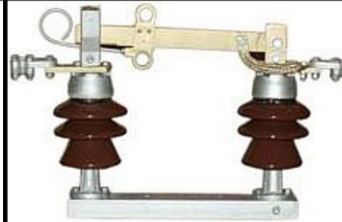
AIR BREAK SWITCH (33 KV - Tilting type)
